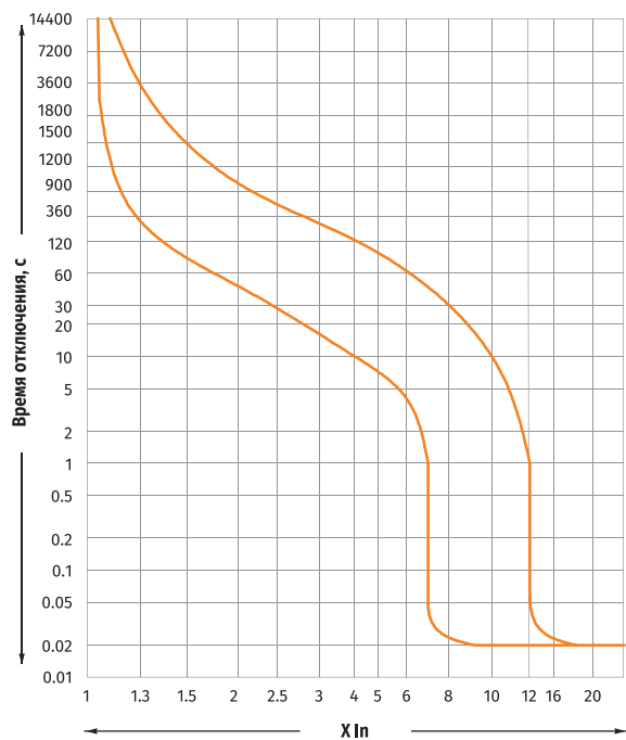
BA88-36/400, 300-400 A
